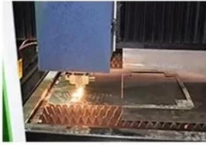
Laser cutting
